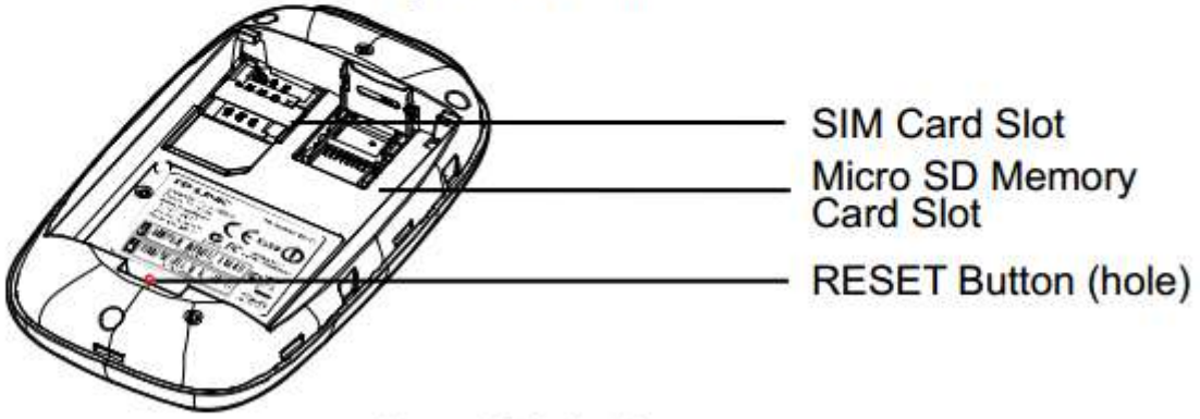
Figure 1-2 the Interior
